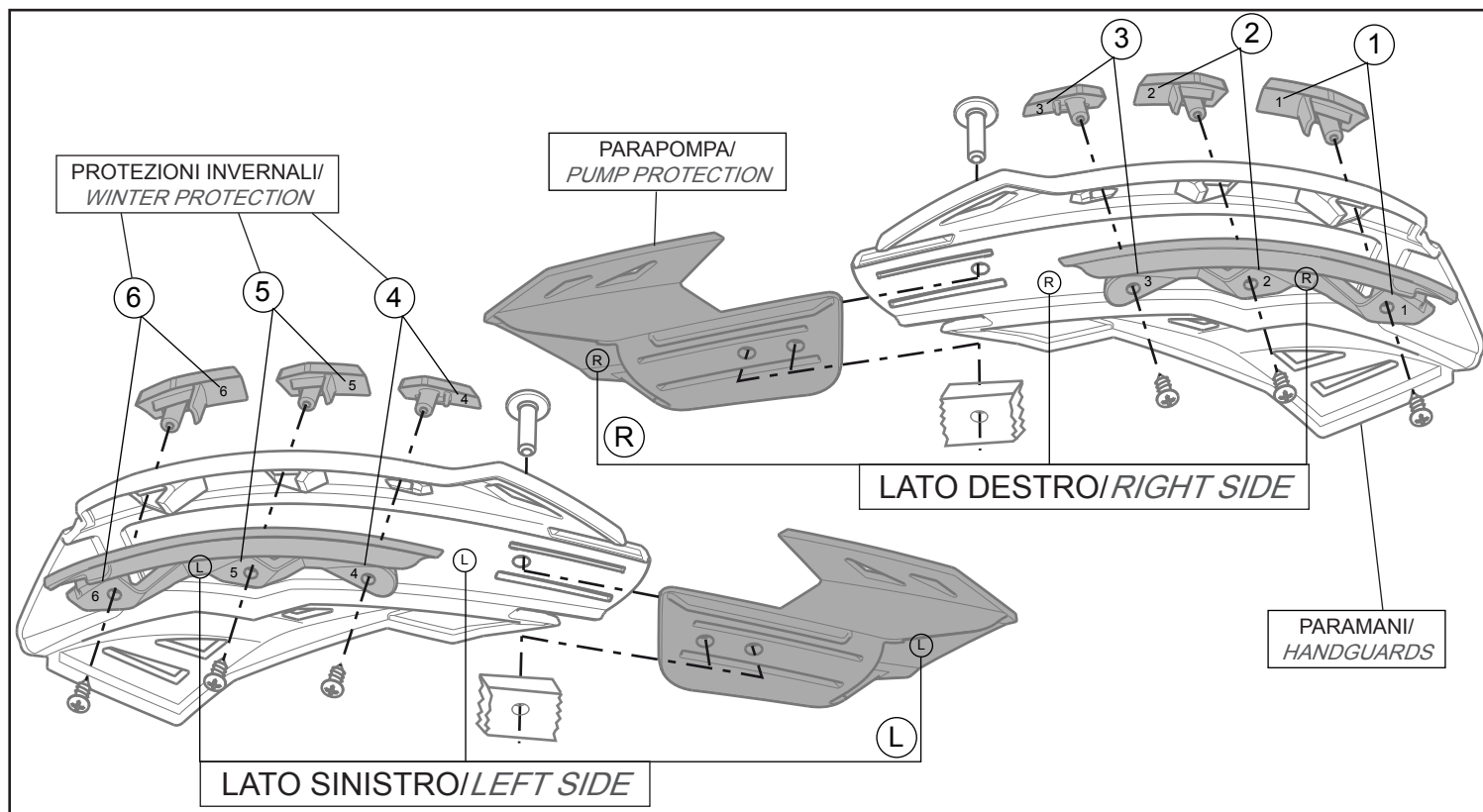
Schema assemblaggio componenti paramani / Handguards components assembly scheme
