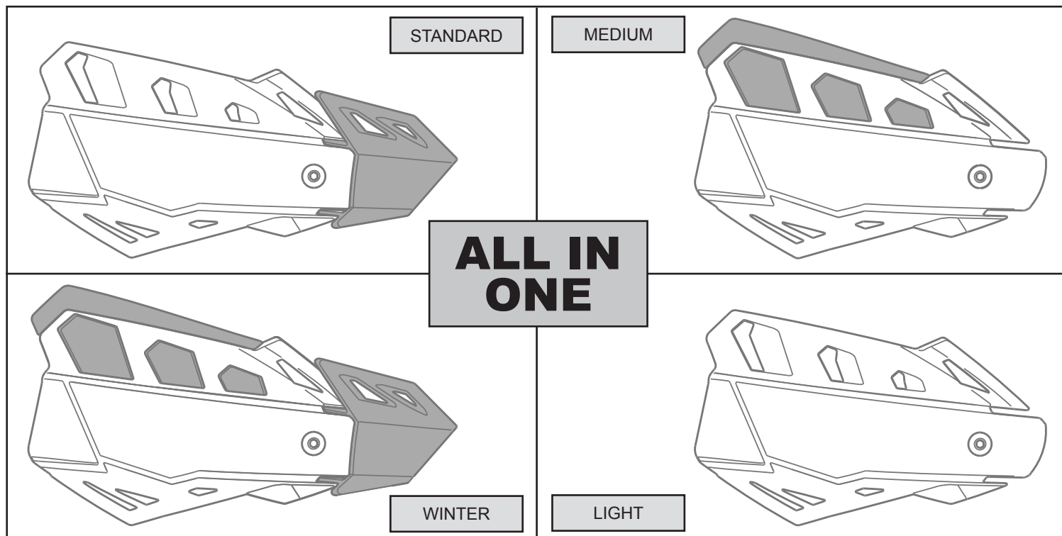
Schema assemblaggio componenti paramani / Handguards components assembly scheme
